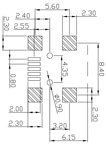
PCB LAYOUT
