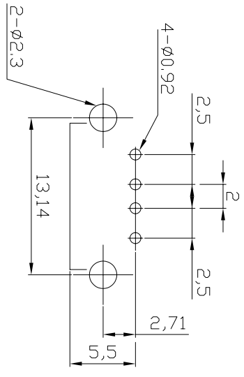
Pin Hole Layout (Jack Bottom View)
